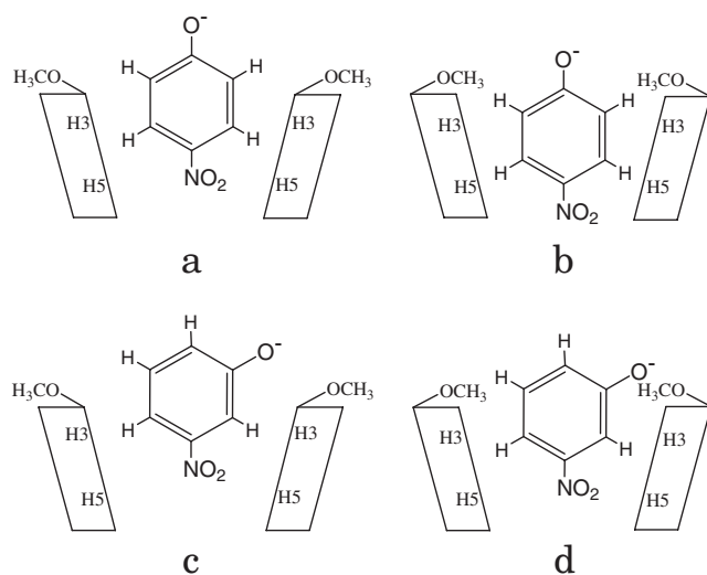
Figure 2. Possible structures of the inclusion complexes of 2α and 3α with p -NP and m -NP in alkaline solutions. (a) 2α - p -NP complex, (b) 3α - p -NP complex, (c) 2α - m -NP complex, (d) 3α - m -NP complex.
