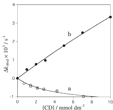
Figure 3. Plots of the difference ( \Delta k_{\text{obsd}} ) between the rates of the cleavage of m -NPA in the presence ( k_{\text{obsd}} ) and in the absence ( k_{\text{un}} ) of the permethylated CDs vs. CD concentration in a carbonate buffer (pH 10.60) at 298 K. Permethylated CDs added are 2α (a) and 3α (b), respectively.
