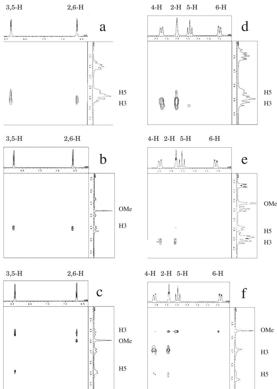
Figure 1. ROESY spectra of p -NP or m -NP in the presence of \alpha -CD, 2 \alpha , or 3 \alpha in D 2 O containing 0.1 mol dm -3 Na 2 CO 3 at 298 K. (a) 10.2 mmol dm -3 p -NP + 42.0 mmol dm -3 \alpha -CD, (b) 10.1 mmol dm -3 p -NP + 13.8 mmol dm -3 2 \alpha , (c) 10.1 mmol dm -3 p -NP + 12.9 mmol dm -3 3 \alpha , (d) 10.2 mmol dm -3 m -NP + 31.6 mmol dm -3 \alpha -CD, (e) 10.2 mmol dm -3 m -NP + 16.9 mmol dm -3 2 \alpha , (f) 10.2 mmol dm -3 m -NP + 13.4 mmol dm -3 3 \alpha .
